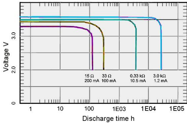
Continuous discharge at 25°C
